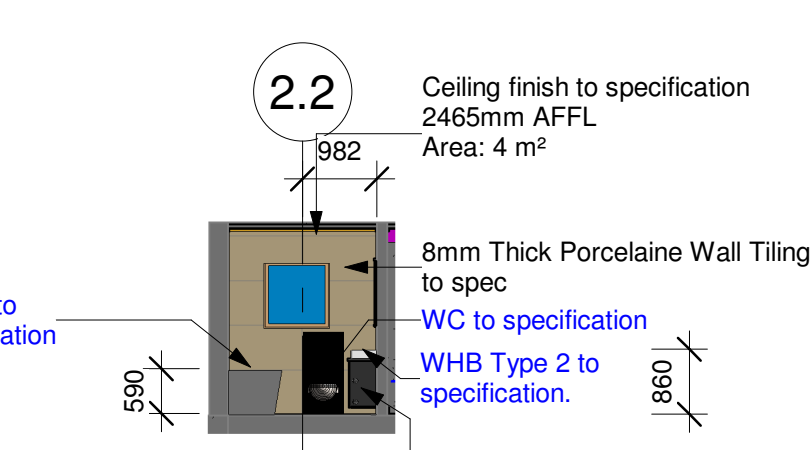
2.2 Ceiling finish to specification 2465mm AFFL Area: 4 m 2 8mm Thick Porcelaine Wall Tiling to spec WC to specification WHB Type 2 to specification. Vanity Type 2 to specification By nominated supplier
