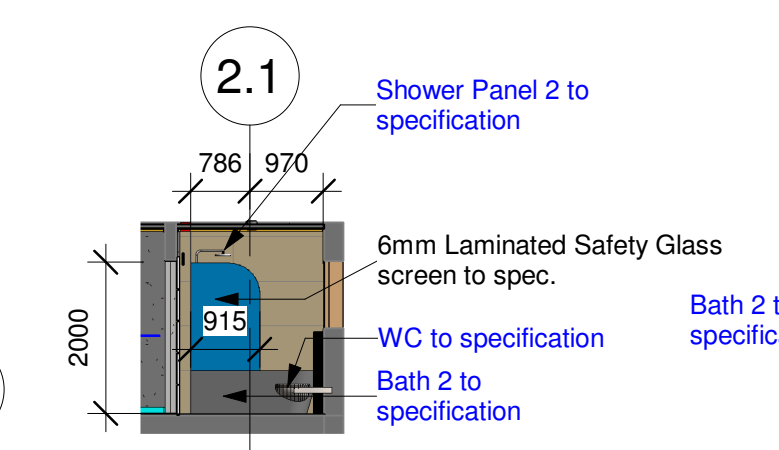
2.1 Shower Panel 2 to specification 6mm Laminated Safety Glass screen to spec. WC to specification Bath 2 to specification
