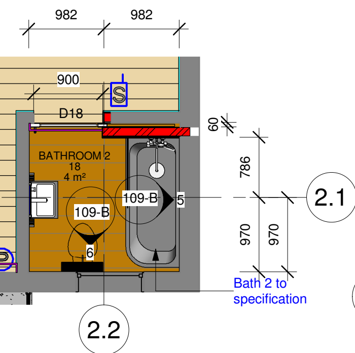
4 FIRST FLOOR - Bathroom 2 1 : 50
