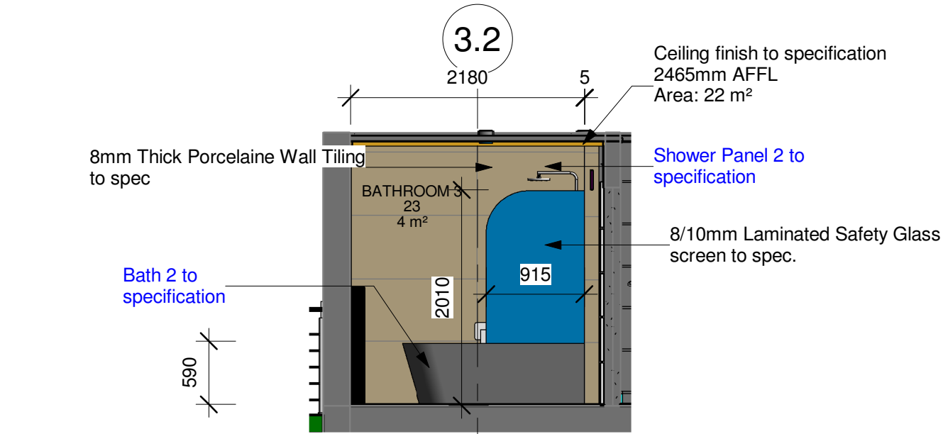
Elevation Bathroom 3.2
