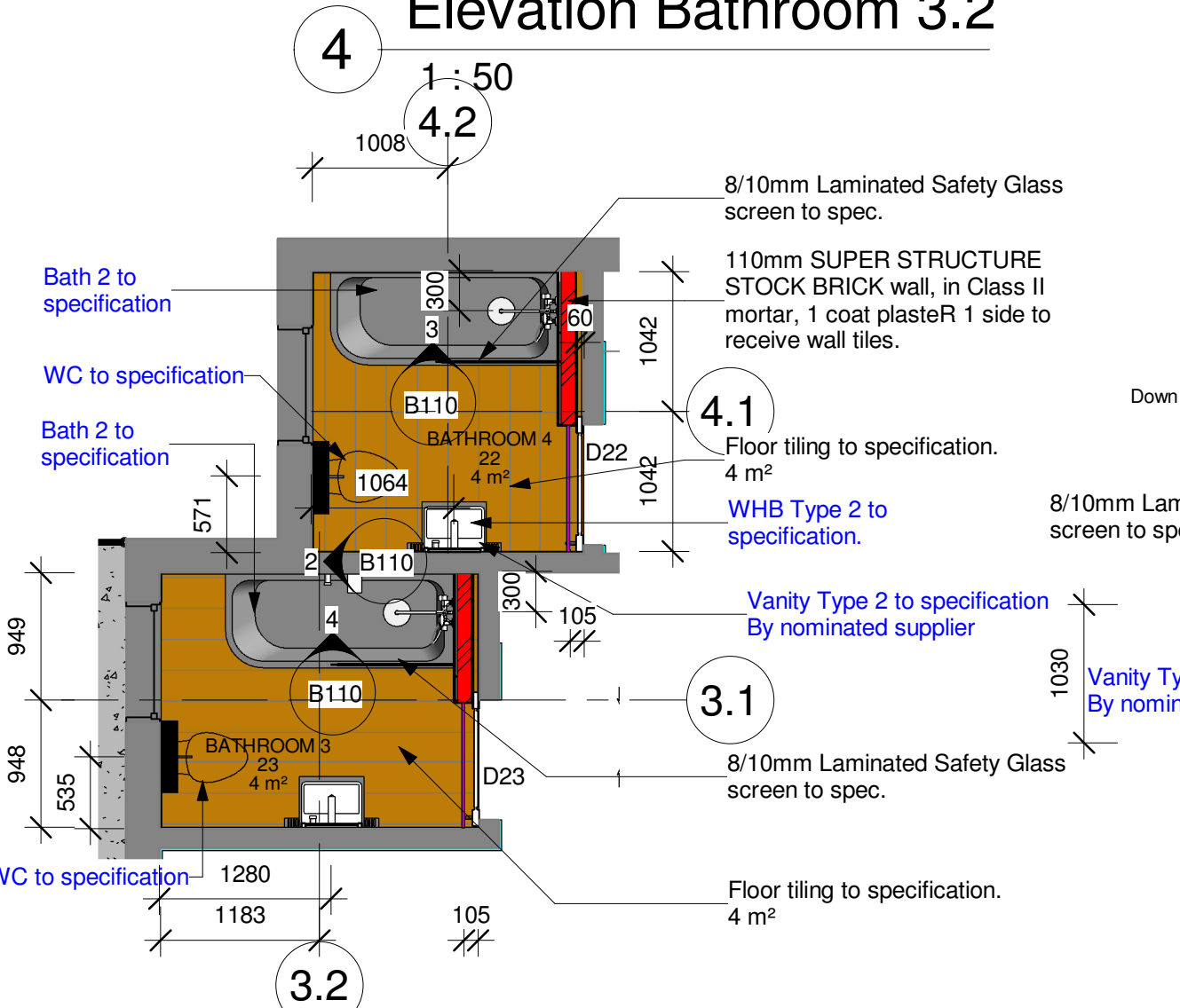
FIRST FLOOR - Bathrooms 3 & 4
