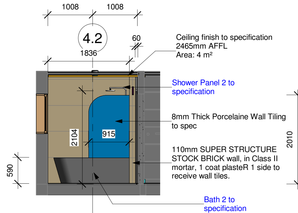
Elevation Bathroom 4.2
